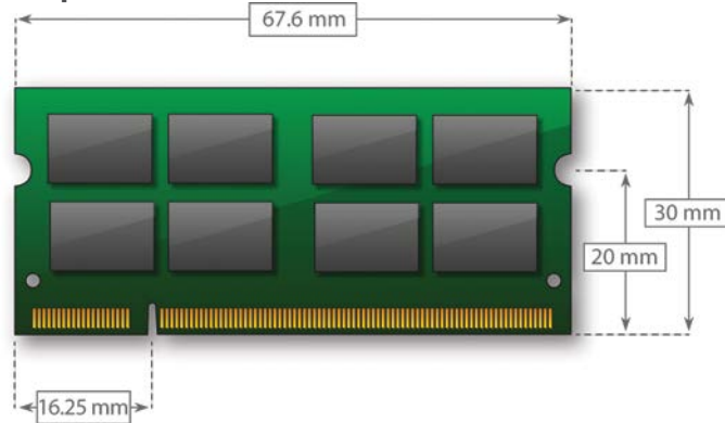
DDR2 SO-DIMM (200 pin)
