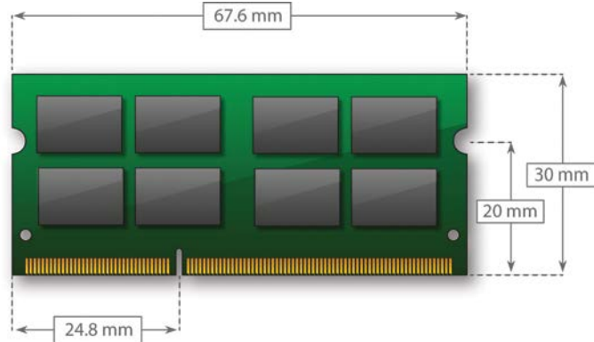
DDR3 SO-DIMM (204 pin)
