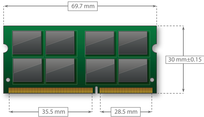
DDR3 SO-DIMM (204 pin)
