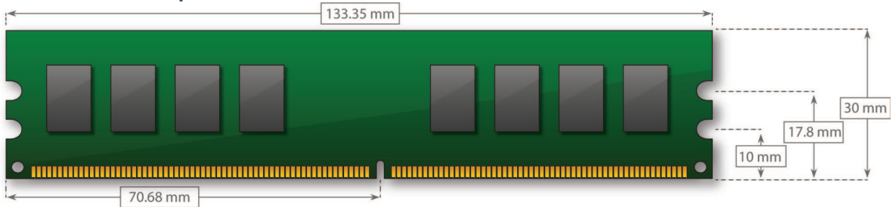
DDR2 FULLY BUFFERED DIMM (240 pin)
