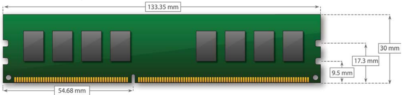
DDR3 DIMM (240 pin)
