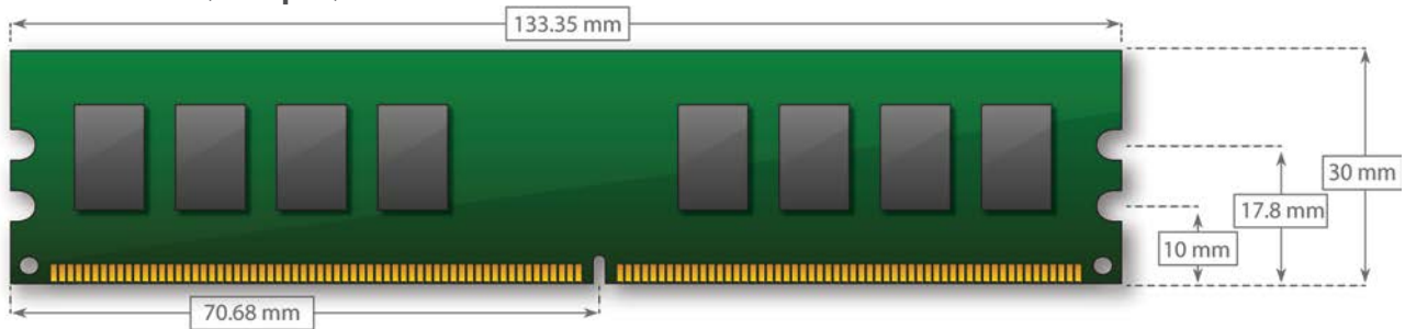
DDR2 DIMM (240 pin)
