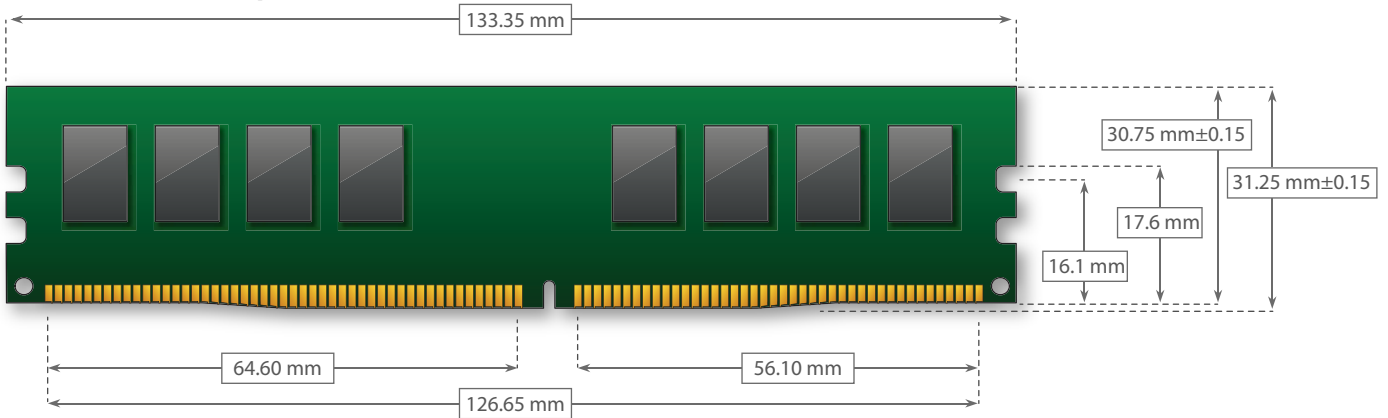
DDR4 DIMM (288 pin)
