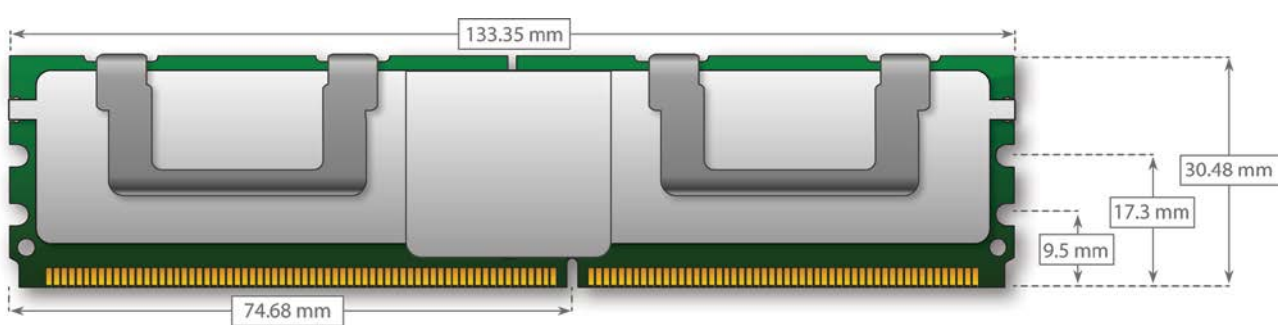
DDR2 FULLY BUFFERED DIMM (240 pin)
